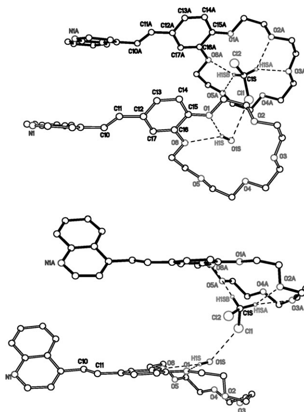
Fig. 15 Two projections of two adjacent molecules of 3 in a staircase; the additional 'A' letter indicates that atoms are at ( x , 1 + y , z ). Hydrogen bonds are shown as dashed lines. Hydrogen atoms of 3 that are not involved in secondary interactions are omitted for clarity.
