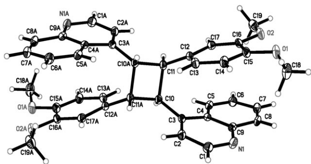
Fig. 11 The structure of compound 6 obtained after 30 h irradiation of 1 ; the additional letter 'A' indicates that atoms are at (2 - x, 2 - y, 1 - z) . Thermal ellipsoids are drawn at the 50% probability level.
