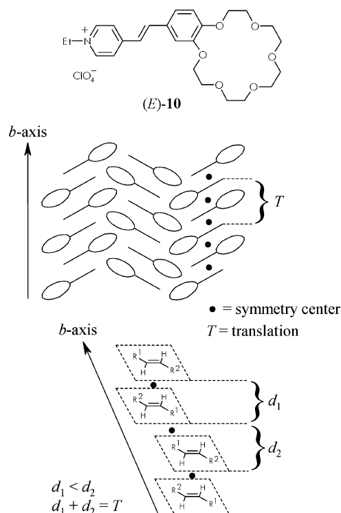
Scheme 4 Structure of dye 10 (above), its crystal packing (middle) and a schematic showing the structure of a stack of molecular sandwiches (below).
