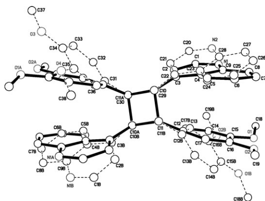
Fig. 13 Superposition of cyclobutane units in 6 (full lines) and 6 · 2HClO 4 (dashed lines). All hydrogen atoms are omitted for clarity.
