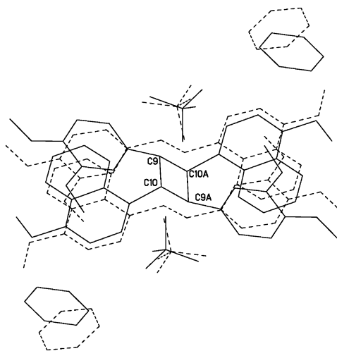
Fig. 6 Superposition of the same areas of crystal unit cell for 2 (dashed lines) and 7 (solid lines); the additional letter 'A' indicates that atoms are at (1 - x, 1 - y, 1 - z) .
