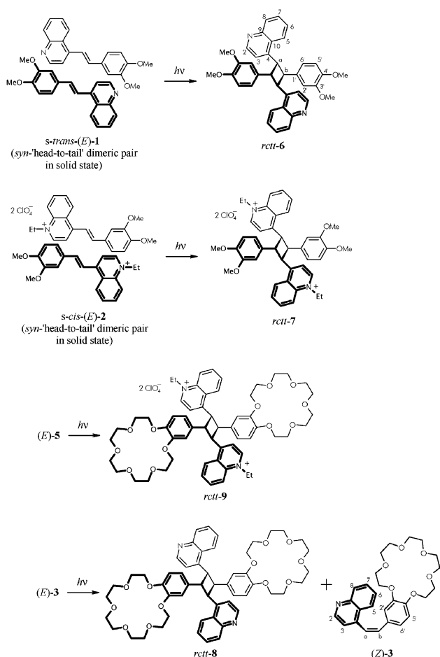
Scheme 3 Solid-phase synthetic routes for the formation of cyclobutanes rctt -6–9.
