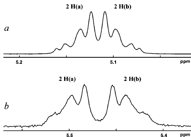
Fig. 1 The ^1\text{H} NMR spectra (region of the cyclobutane protons) in \text{DMSO}-d_6 at 25^\circ\text{C} : (a) the product of the photoirradiation of (E)-1 as a thin film for 20 h ( rectt-6 ); (b) product of the photoirradiation of (E)-2 as a thin film for 35 h ( rectt-7 ).
