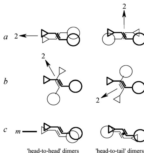
Scheme 7 Possible mutual arrangements of styryl dye molecules in dimeric pair. Here circles denote phenyl substituents and triangles are heterocyclic moieties.
