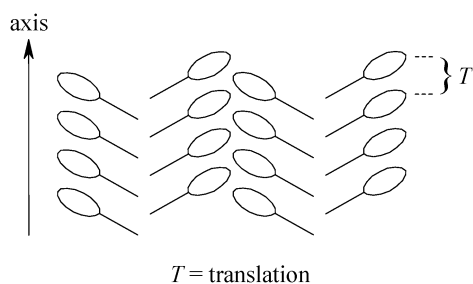
Scheme 5 'Head-to-head' crystal packing motif.
