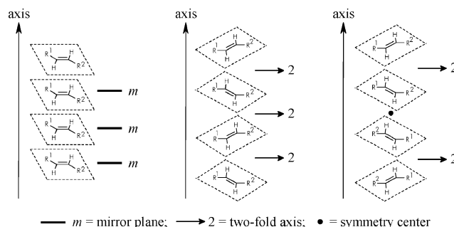
Scheme 6 Stacks of unsaturated molecules formed via mirror planes (left side), two-fold axes (middle), and a combination of a two-fold axis with symmetry center (right side).
