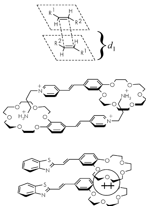
Scheme 1 The precursor dimer for the PCA reaction, and examples of the self-assembly in solution of two crown-ether stilbene-like molecules.
