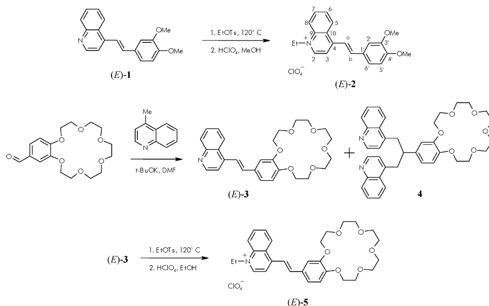
Scheme 2 The synthetic route affording 4-styrylquinoline compounds 2 , 3 , 5 and the bisheterocycle 4 .
