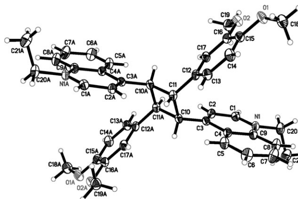
Fig. 7 The structure of rectt-7a ; the additional 'A' letter indicates that atoms are at (1 - x, -y, 1 - z) .
