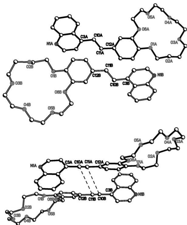
Fig. 16 Two centrosymmetrically related molecules of 3 in different projections; the additional letter 'B' indicates that atoms are at (2 - x, 1 - y, 1 - z) . All hydrogen atoms and solvate molecules are omitted for clarity.
