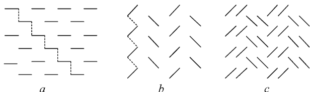
Scheme 8 Packing motifs in crystals of 1-hetaryl-2-phenylethylenes: staircase ( a ), parquet ( b ), and parquet sandwich ( c ). Solid lines denote the profiles of the conjugated fragments of the molecules.
