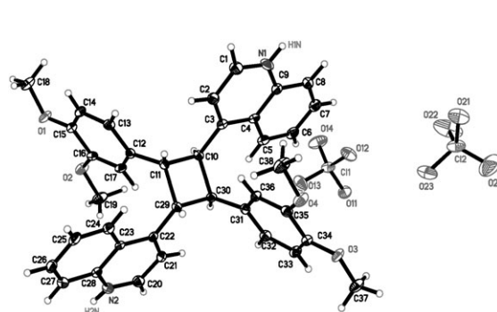
Fig. 12 The structure of 6 ·2HClO 4 . Thermal ellipsoids are drawn at the 50% probability level.
