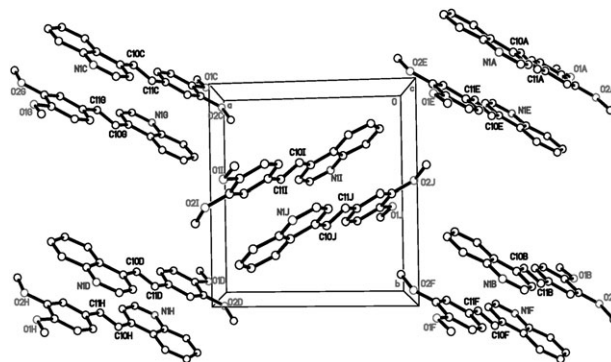
Fig. 9 A fragment of crystal packing of 1 .
