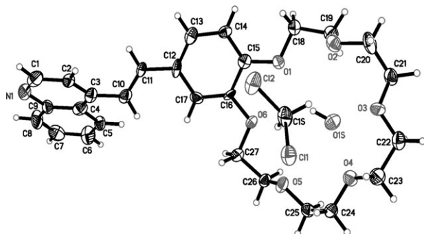
Fig. 14 The structure of 3 . Thermal ellipsoids are drawn at the 50% probability level.
