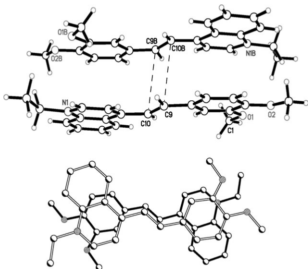
Fig. 4 Structure of a sandwich of 2 in two projections. In the below projection the upper molecule is drawn with hollow lines, and all hydrogen atoms are omitted for clarity; the additional letter 'B' indicates that atoms are at (1 - x, 1 - y, 1 - z) .
