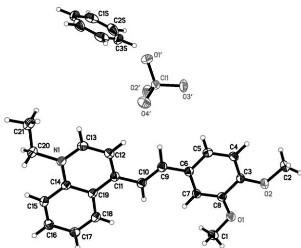
Fig. 2 Structure of compound 2 . Thermal ellipsoids are drawn at the 50% probability level.
