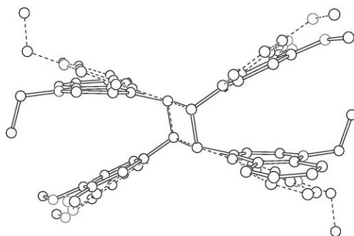
Fig. 8 Superposition of the cyclobutane molecules in 7 (hollow lines) and 7a (dashed lines).
