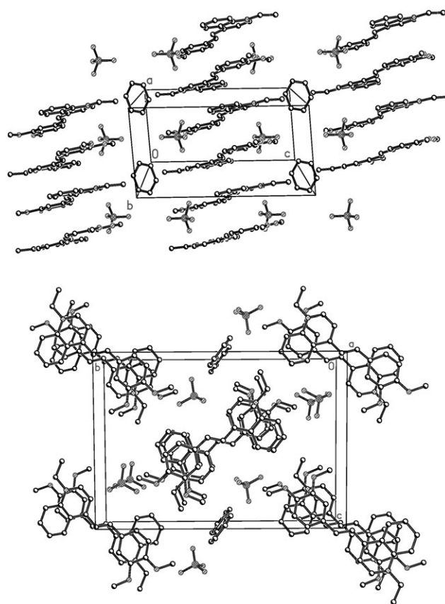
Fig. 3 Crystal packing of 2 as viewed down the b axis (above) and down the a axis (below).
