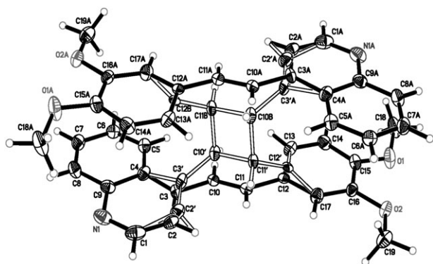
Fig. 10 The X-ray structure of 1/6 obtained after 6 h irradiation of 1 . The atoms belonging to 6 are connected by hollow lines; the additional letter 'A' or 'B' indicates that atoms are at (3 - x, 1 - y, 1 - z) . The thermal ellipsoids are drawn at the 50% probability level.
